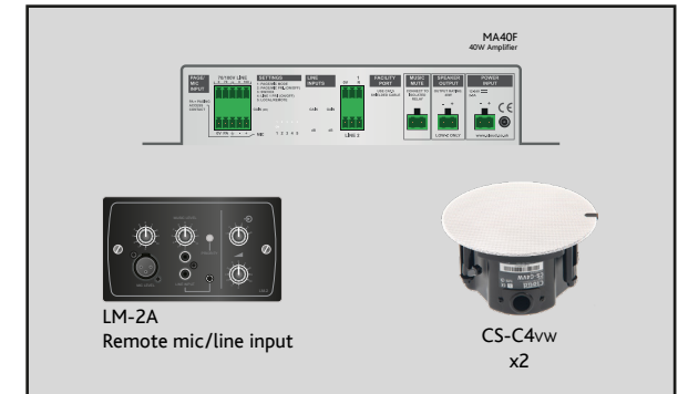
Zone: 8 (Independent) - Meeting Room.
