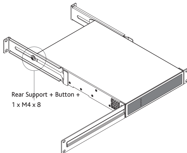
Diagram 4B CXA with rack support hardware. 2 positions.
