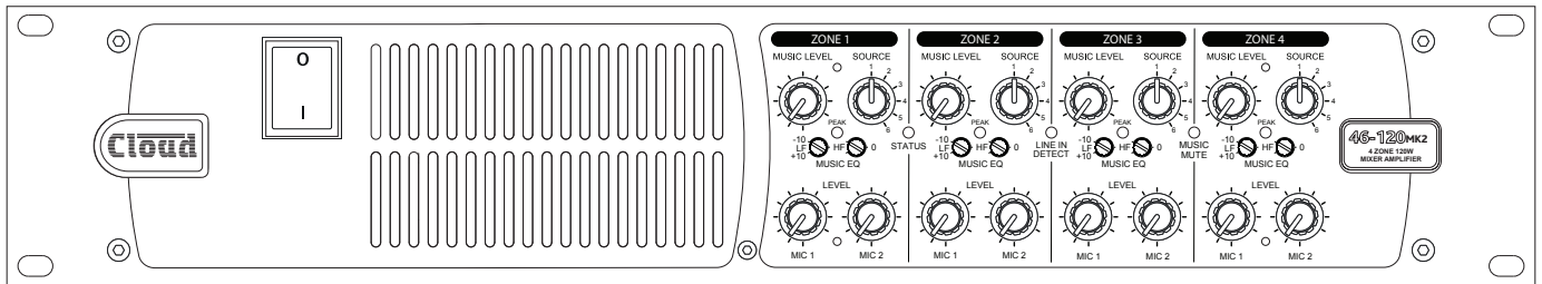
Front panel view (46-120MK2 illustrated)
