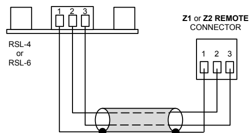
REMOTE SOURCE & LEVEL CONTROL WIRING
